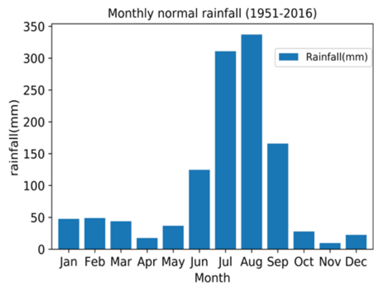
Figure 3.1: Monthly normal accumulated rainfall (1951–2016)
