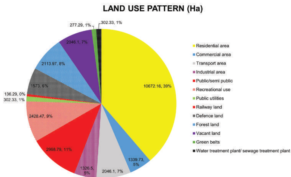
Figure 2.5: Category wise distribution of Land Use Pattern in Chandigarh
