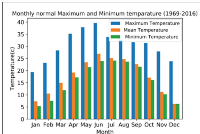
Figure 3.10: Monthly mean temperature over Chandigarh (1969–2016)
