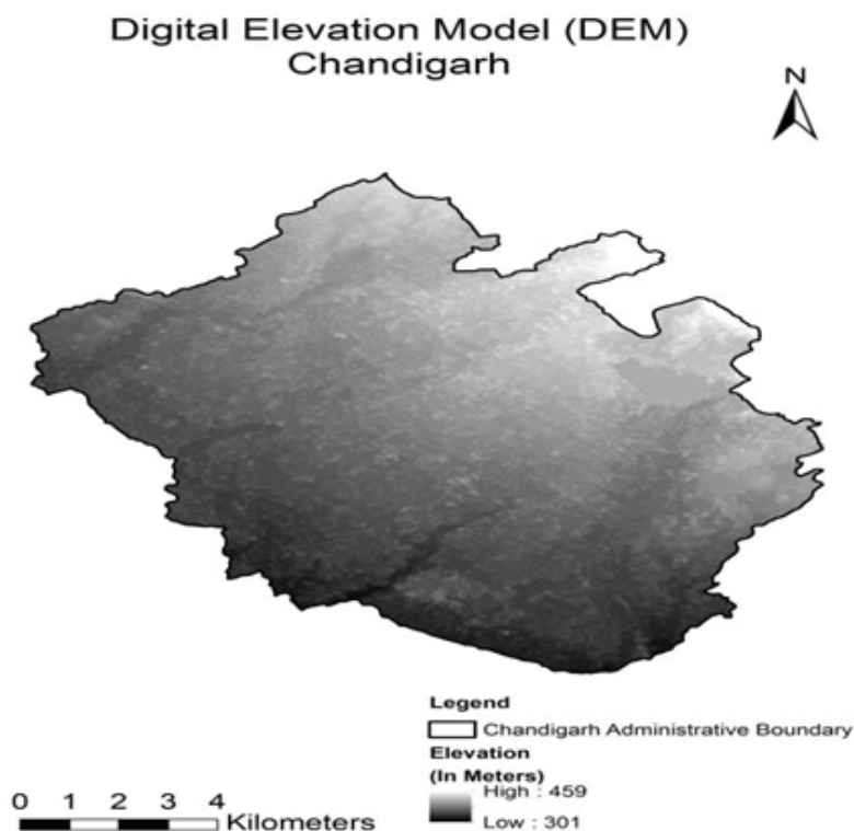
Figure 4.1: Digital Elevation Model of Chandigarh
