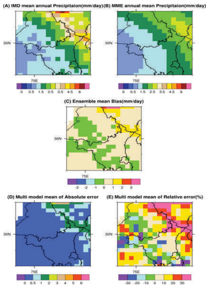
Figure 3.13: (a) Annual climatological (1976–2005) mean precipitation (mm) from IMD observations, (b) NEX-GDDP multi-model ensemble mean annual climatological (1976–2005) mean precipitation (mm), (c) bias (IMD-MME) in NEX-GDDP rainfall (mm) with respect to IMD observations, (d) absolute error in NEX-GDDP rainfall (mm) with respect to IMD observations, and (e) relative error in NEX-GDDP rainfall (%) with respect to IMD observations
